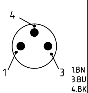
MALE END VIEW
